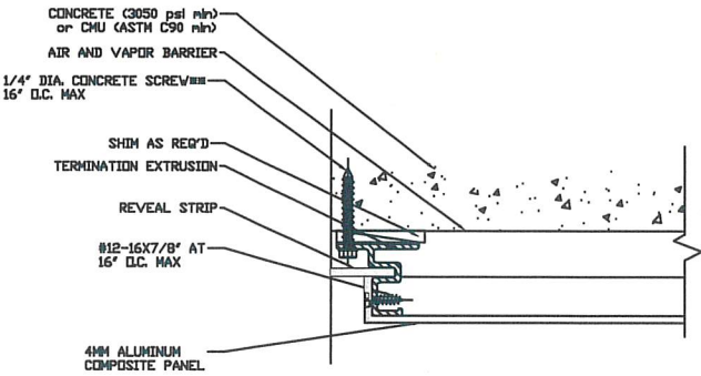
4A JAMB TERMINATION REF: NONE (HEAD AND SILL ARE SIMILAR) SCALE: 6"=1'-0"
