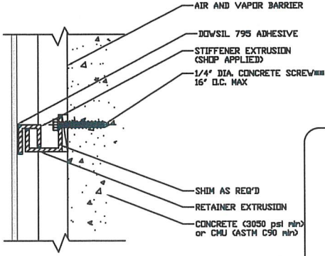
6A STIFFENER/RETAINER DETAIL REF: NONE SCALE: 6"=1'-0"
