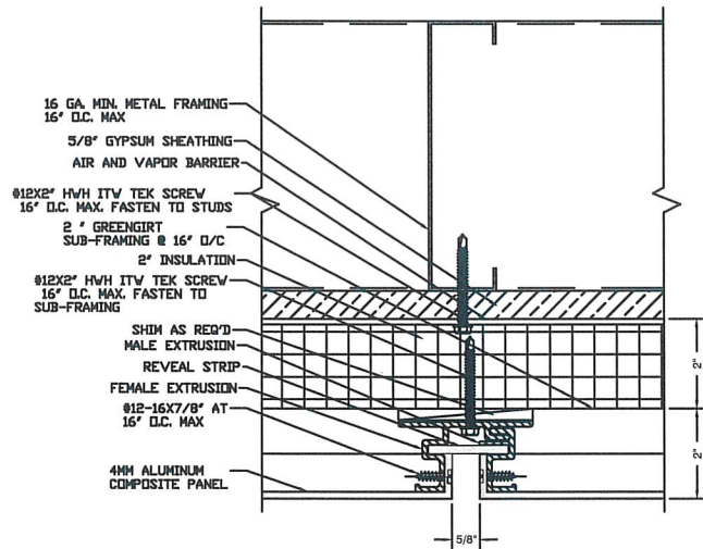
5 TYP. VERTICAL JOINT REF: NONE SCALE: 6"=1'-0"
