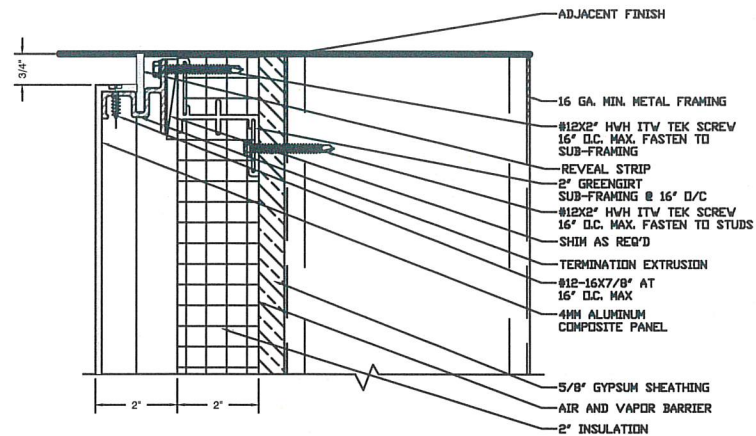
1 HEAD TERMINATION REF: NONE SCALE: 6"=1'-0"
