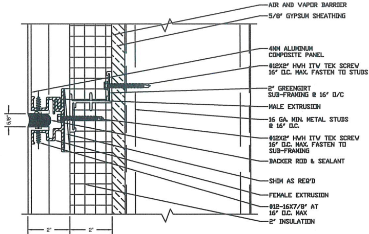
2 3.3 TYP. HORIZONTAL JOINT REF: NONE SCALE: 6"=1'-0"
