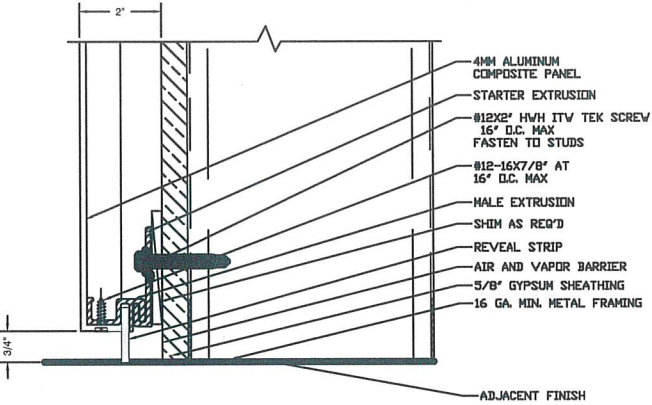
3 TYP. BASE TERMINATION REF: NONE SCALE: 6"=1'-0"
