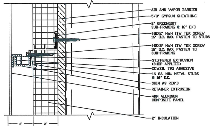
6 3.3 STIFFENER/RETAINER DETAIL REF: NONE SCALE: 6"=1'-0"
