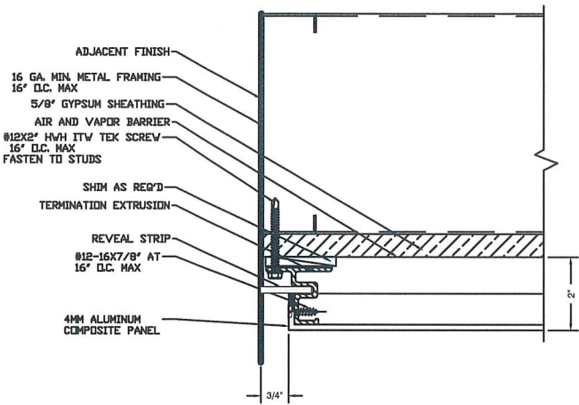
4 JAMB TERMINATION REF: NONE SCALE: 6"=1'-0"
