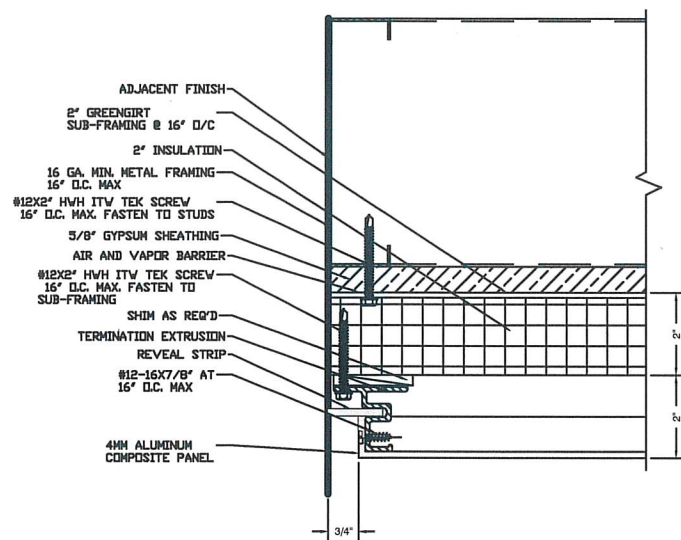
4 JAMB TERMINATION REF: NONE SCALE: 6"=1'-0"
