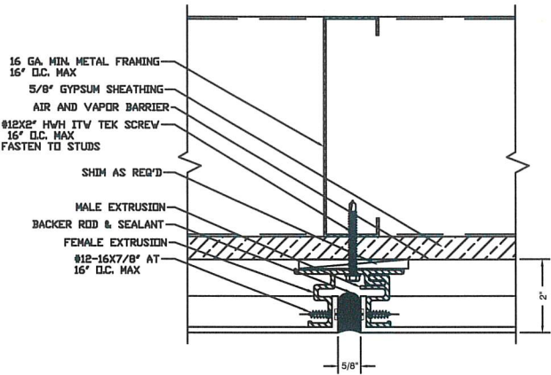
5 TYP. VERTICAL JOINT 3.1 REF: NONE SCALE: 6"=1'-0"
