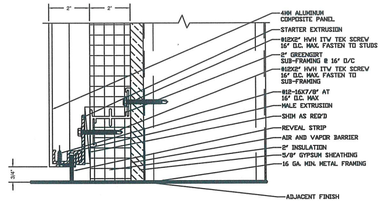
3 TYP. BASE TERMINATION REF: NONE SCALE: 6"=1'-0"
