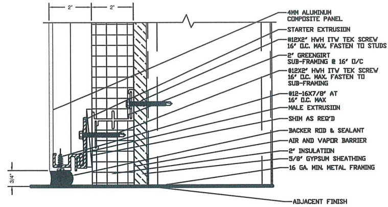
3 3.3 TYP. BASE TERMINATION REF: NONE SCALE: 6"=1'-0"
