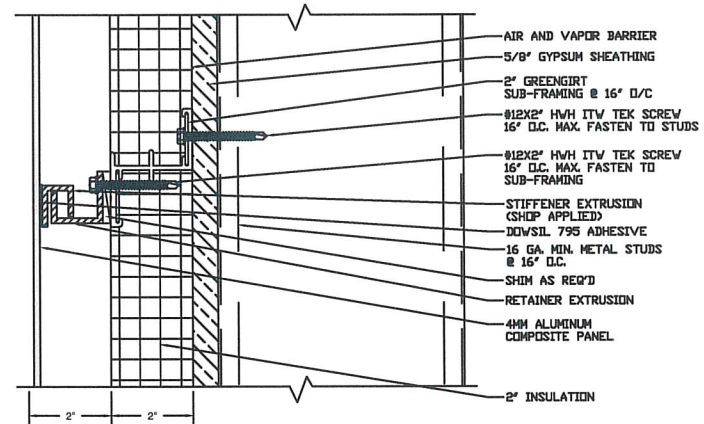
6 STIFFENER/RETAINER DETAIL REF: NONE SCALE: 6"=1'-0"
