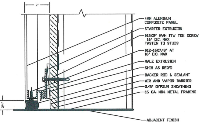
3 TYP. BASE TERMINATION 3.1 REF: NONE SCALE: 6"=1'-0"
