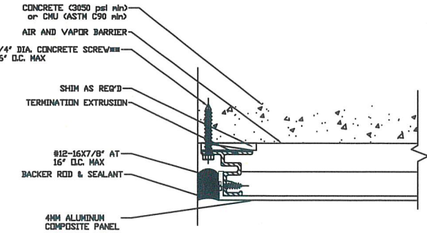
4A JAMB TERMINATION 3.1 REF: NONE (HEAD AND SILL ARE SIMILAR) SCALE: 6"=1'-0"
