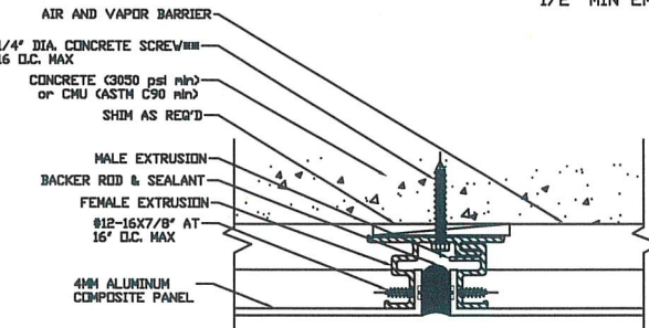
5A TYP. VERTICAL JOINT 3.1 REF: NONE (TYP. HORIZONTAL JOINT IS SIMILAR) SCALE: 6"=1'-0"
