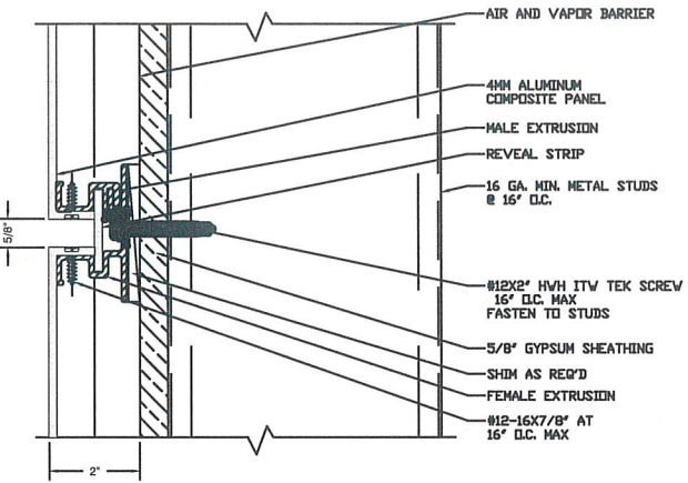
2 TYP. HORIZONTAL JOINT REF: NONE SCALE: 6"=1'-0"
