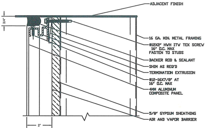
1 HEAD TERMINATION 3.1 REF: NONE SCALE: 6"=1'-0"
