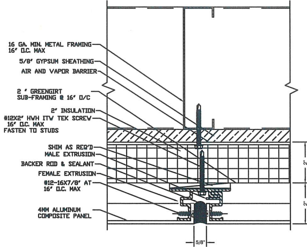
5 3.3 TYP. VERTICAL JOINT REF: NONE SCALE: 6"=1'-0"
