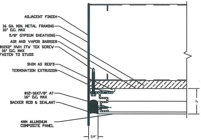
4 JAMB TERMINATION 3.1 REF: NONE SCALE: 6"=1'-0"
