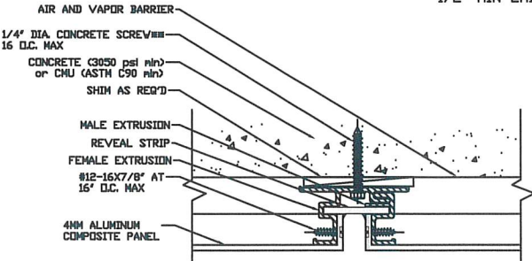
5A TYP. VERTICAL JOINT REF: NONE (TYP. HORIZONTAL JOINT IS SIMILAR) SCALE: 6"=1'-0"
