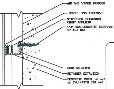
6A STIFFENER/RETAINER DETAIL 3.1 REF: NONE SCALE: 6"=1'-0"
