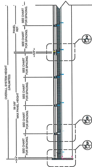
3 2.3 REF: NONE SCALE: 1"=1'-0" PANELS SECTION -B- WET SEAL W. INSULATION AND SUB-FRAMING
